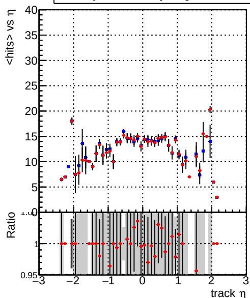
mean hit — DQM_TT_mkFit-DQM_original-0 — DQM_TT_mkFit-DQM_original-127
