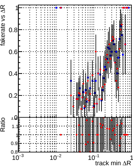
Fake rate vs \Delta R(\text{track, jet}) Legend: DQM_TT_mkFit-DQM_original-0 (blue squares) DQM_TT_mkFit-DQM_original-127 (red circles)
