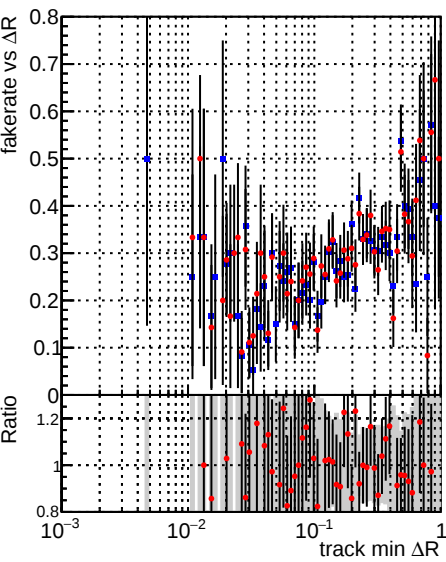
Fake rate vs \Delta R(\text{track, jet}) Legend: DQM_TT_mkFit-DQM_original-0 (blue), DQM_TT_mkFit-DQM_original-127 (red)
