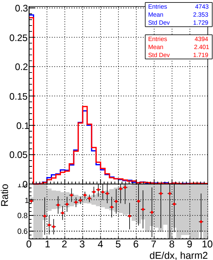
■ DQM_TT_mkFit-DQM_original-0 ● DQM_TT_mkFit-DQM_original-127
