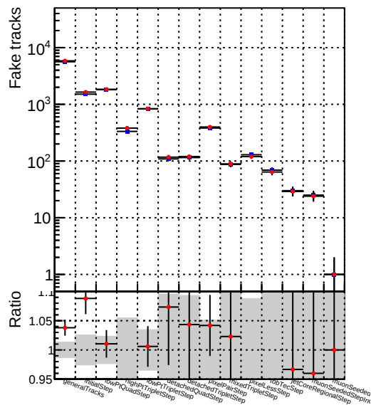
Number —●— DQM_TT_mkFit-DQM_original-127
