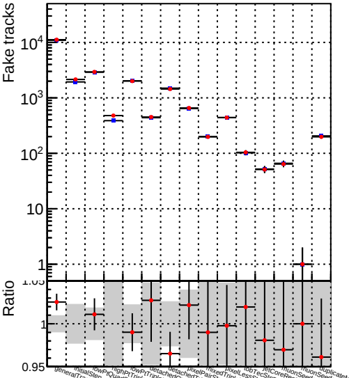
Number —●— DQM_TT_mkFit-DQM_original-127
