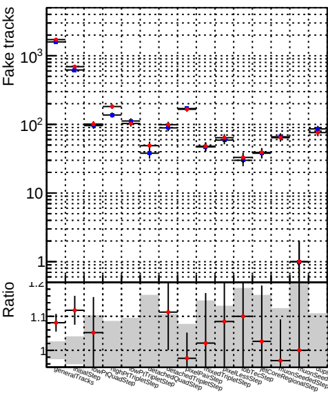
Number —●— DQM_TT__mkFit-DQM_original-127
