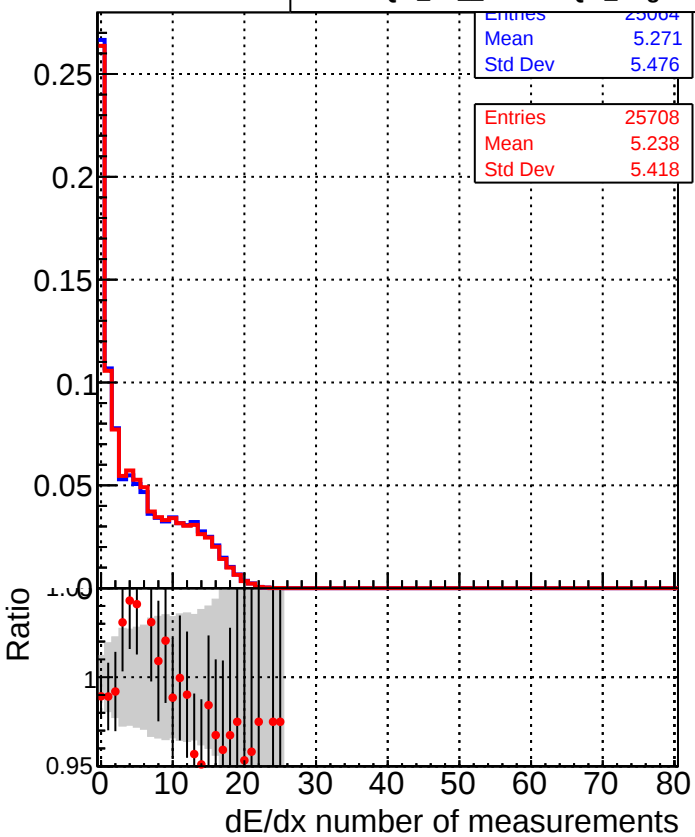
■ DQM_TT_mkFit-DQM_original-0 ● DQM_TT_mkFit-DQM_original-127
