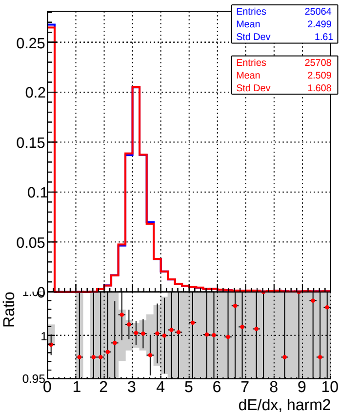
■ DQM_TT_mkFit-DQM_original-0 ● DQM_TT_mkFit-DQM_original-127
