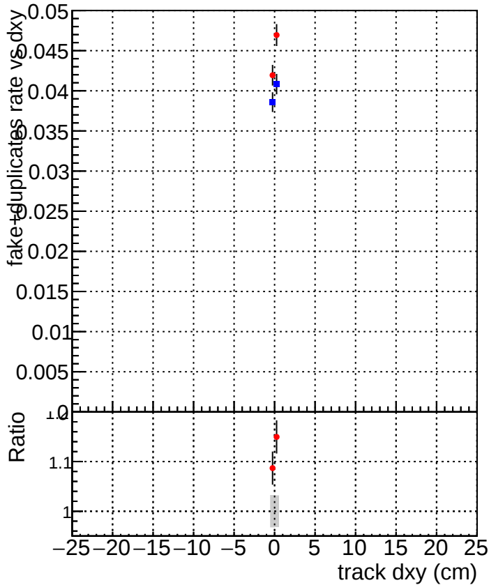
DQM_TT_mkFit-DQM_original-0 DQM_TT_mkFit-DQM_original-127
