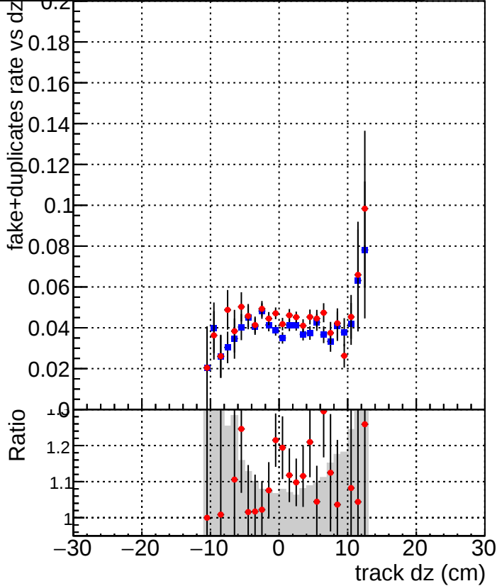
DQM_TT_mkFit-DQM_original-0 DQM_TT_mkFit-DQM_original-127
