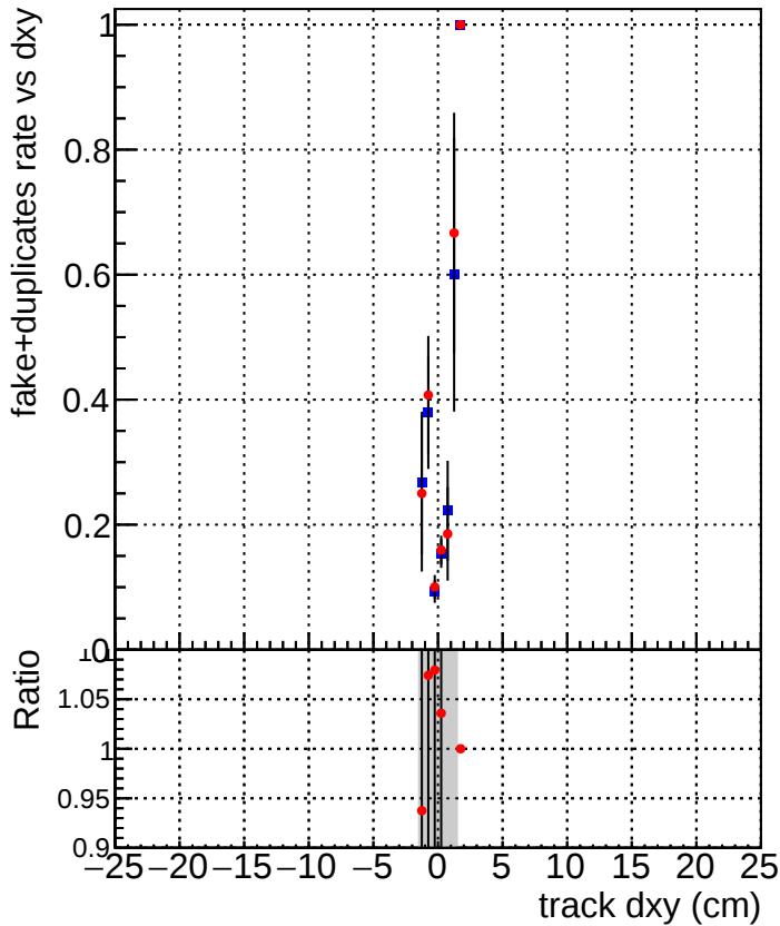
DQM_TT_mkFit-DQM_original-0 DQM_TT_mkFit-DQM_original-127
