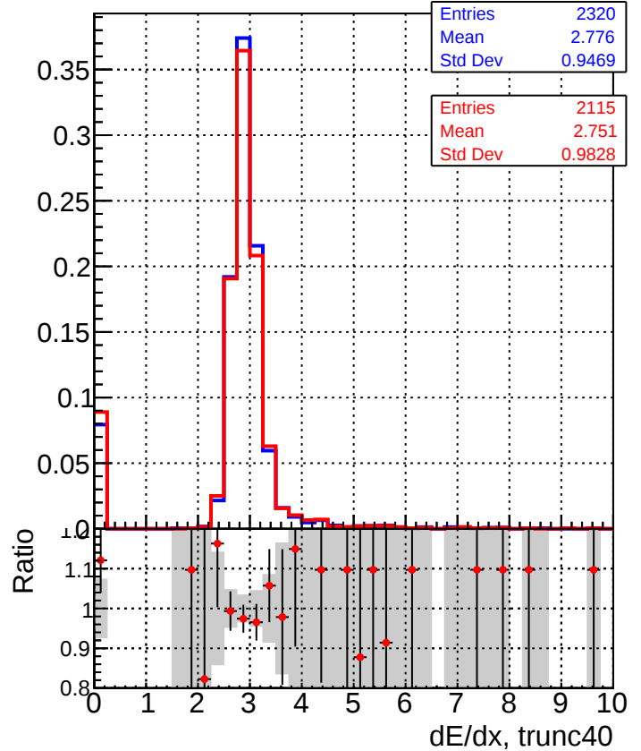
DQM_TT_mkFit-DQM_original-0 DQM_TT_mkFit-DQM_original-127
