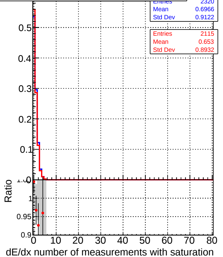
DQM_TT_mkFit-DQM_original-0 DQM_TT_mkFit-DQM_original-127
