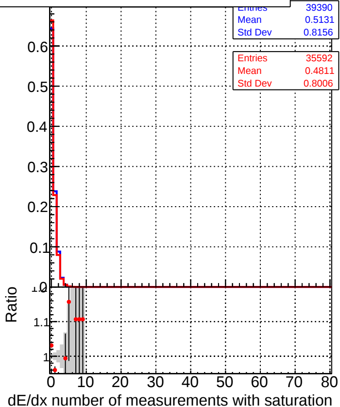
■ DQM_TT_mkFit-DQM_original-0 ● DQM_TT_mkFit-DQM_original-127
