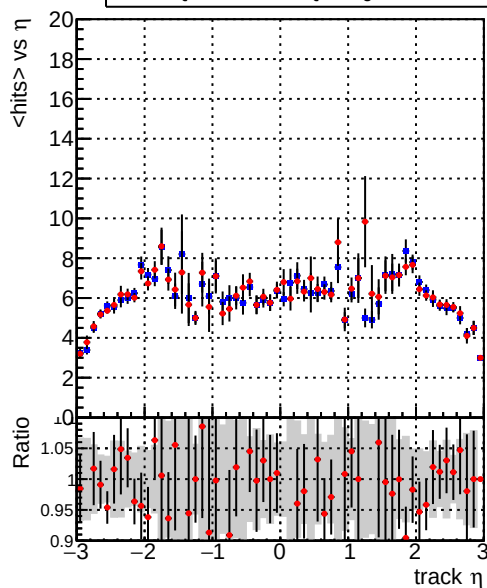
— DQM_TT_mkFit-DQM_original-0 — DQM_TT_mkFit-DQM_original-127
