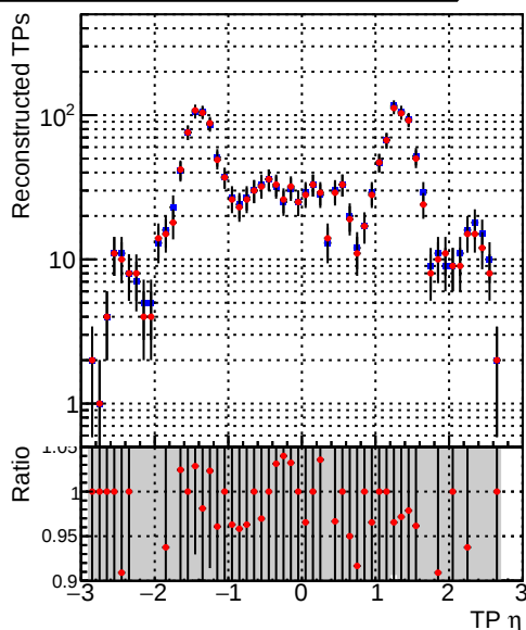
—•— DQM_TT_mkFit-DQM_original-0 —•— DQM_TT_mkFit-DQM_original-127
