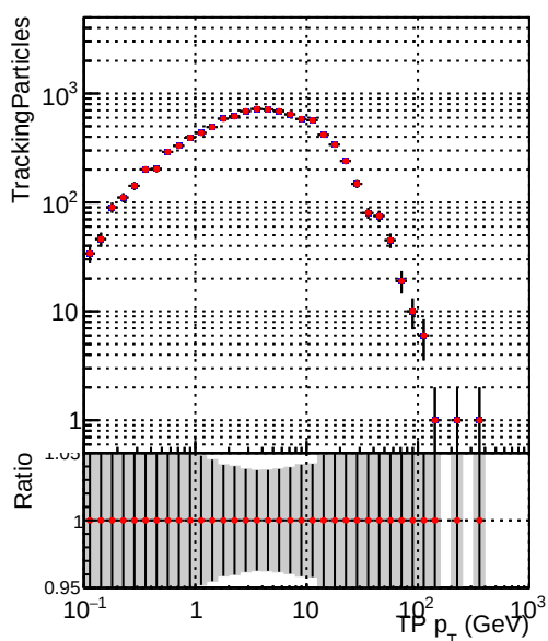
N of simulated tracks vs TP
