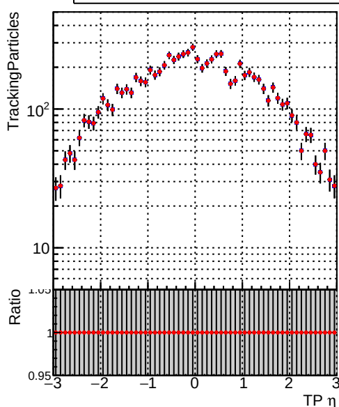
N of simulated tracks vs TP
