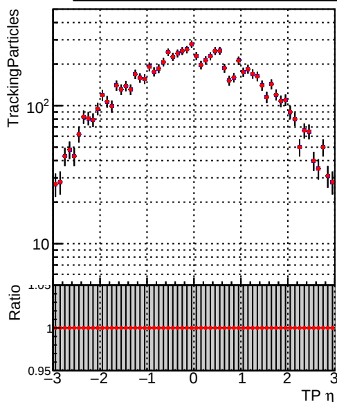
—•— DQM_TT_mkFit-DQM_original-0 —•— DQM_TT_mkFit-DQM_original-127
