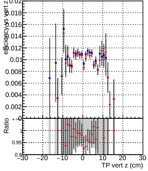
Efficiency vs. sim PV z — DQM_TT_mkFit-DQM_original-0 — DQM_TT_mkFit-DQM_original-127
