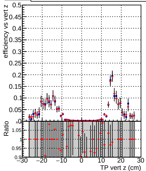
Efficiency vs vert z — DQM_TT_mkFit-DQM_original-0 — DQM_TT_mkFit-DQM_original-127
