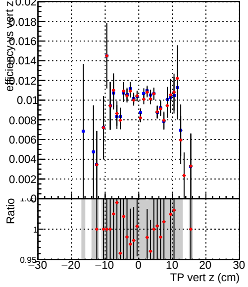
Efficiency vs. TP vert z — DQM_TT_mkFit-DQM_original-0 — DQM_TT_mkFit-DQM_original-127
