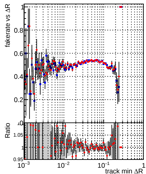
—•— DQM_TT_mkFit-DQM_original-0 —•— DQM_TT_mkFit-DQM_original-127
