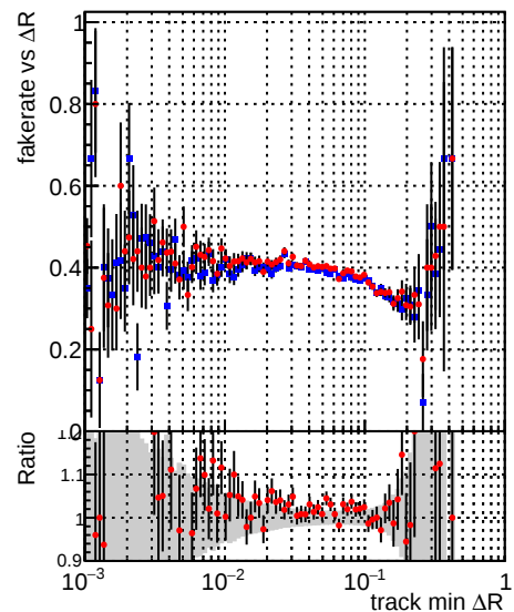
—•— DQM_TT_mkFit-DQM_original-0 —•— DQM_TT_mkFit-DQM_original-127
