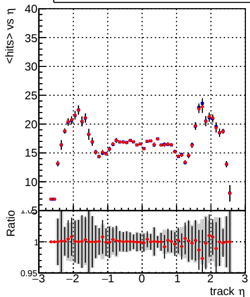
mean hits Legend: DQM_TT_mkFit-DQM_original-0 (blue line), DQM_TT_mkFit-DQM_original-127 (red line)
