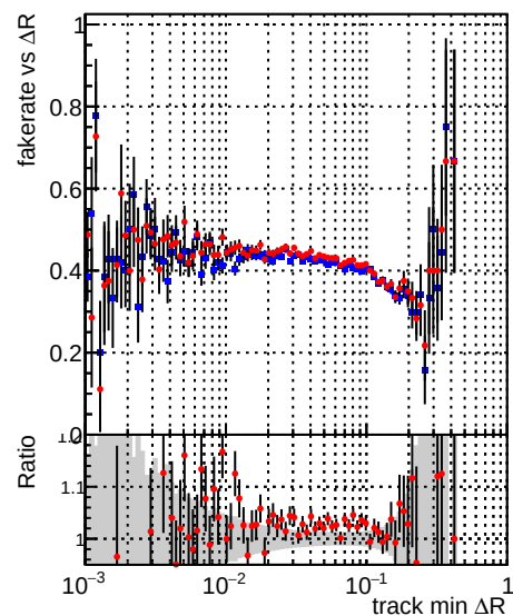
—●— DQM_TT_mkFit-DQM_original-0 —●— DQM_TT_mkFit-DQM_original-127
