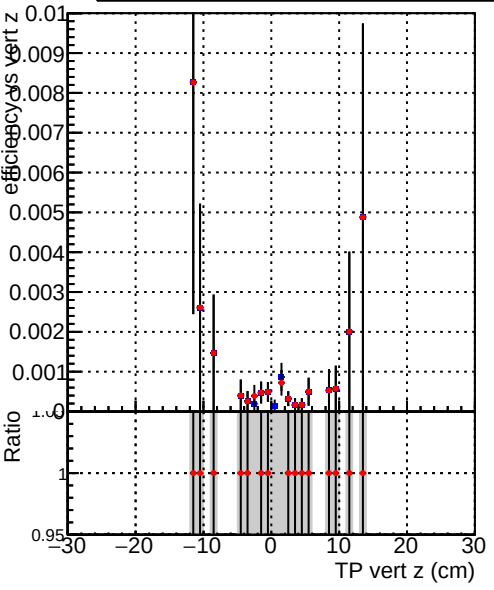
Efficiency vs TP vert z Legend: DQM_TT_mkFit-DQM_original DQM_TT_mkFit-DQM_updated
