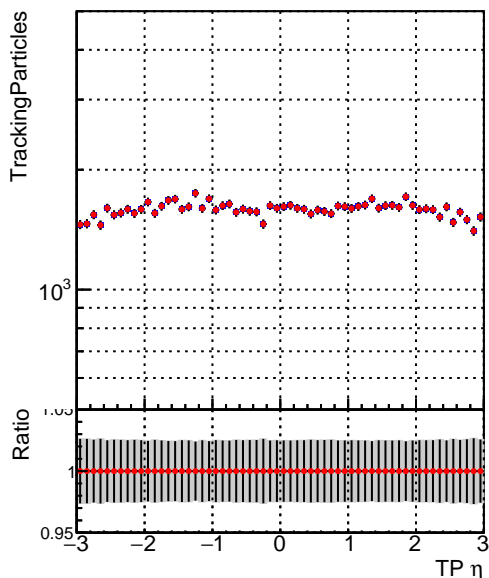
—■ DQM_TT_mkFit-DQM_original —● DQM_TT_mkFit-DQM_updated
