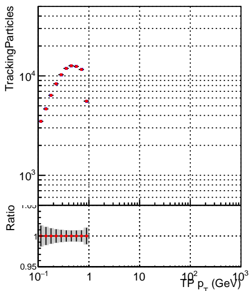
—■ DQM_TT_mkFit-DQM_original —● DQM_TT_mkFit-DQM_updated
