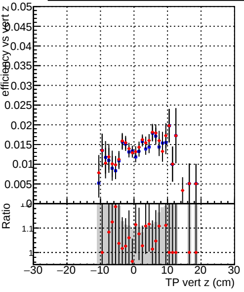
Efficiency vs vertpos Legend: DQM_TT_mkFit-DQM_original DQM_TT_mkFit-DQM_updated
