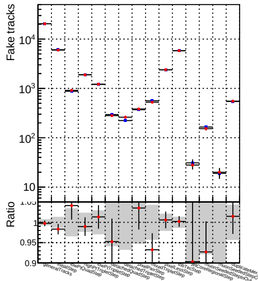
Number —●— DQM_TT__mkFit-DQM_updated
