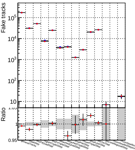
Number —●— DQM_TT_mkFit-DQM_updated
