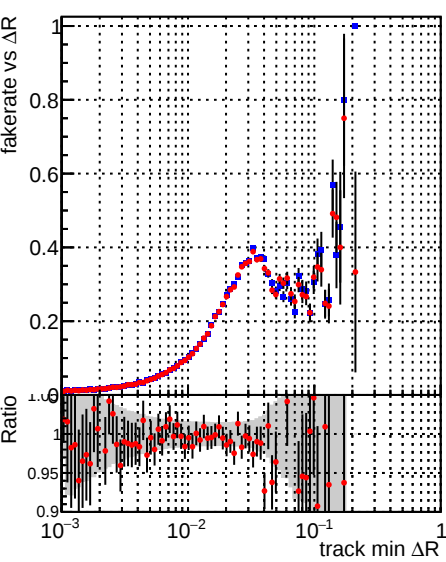
Fake rate vs \Delta R (track, jet) DQM_TT_mkFit-DQM_original DQM_TT_mkFit-DQM_updated
