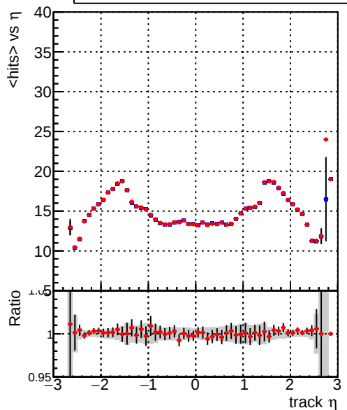
mean hits vs \eta Legend: DQM_TT_mkFit-DQM_original (blue line), DQM_TT_mkFit-DQM_updated (red line)
