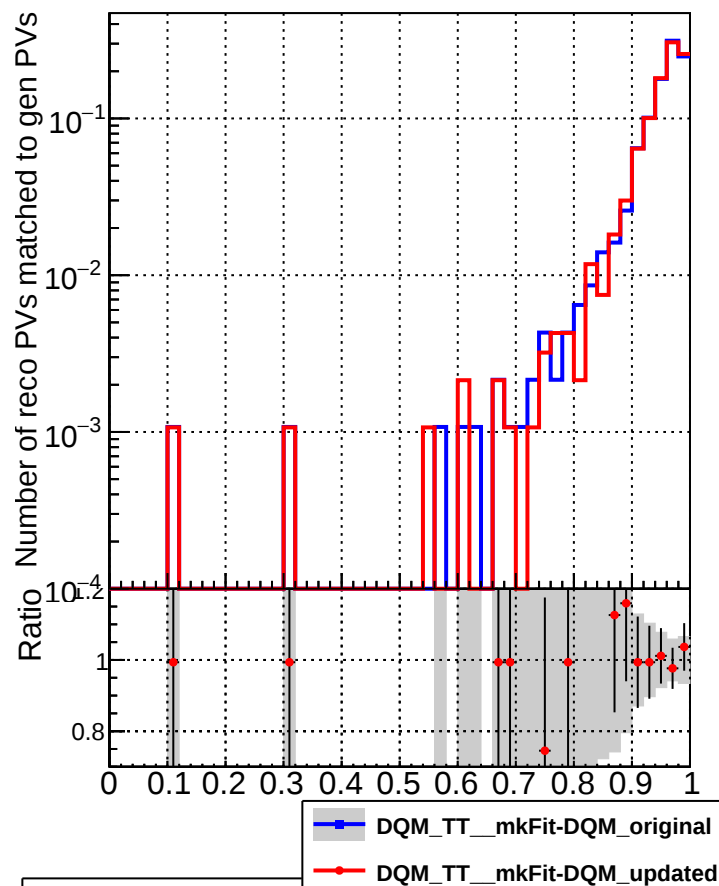
RecoPVAssoc2GenPVmatched_missing
