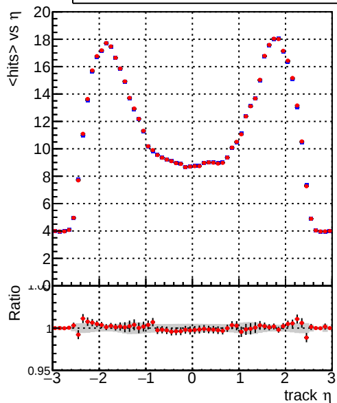
mean hits — DQM_TT_mkFit-DQM_original — DQM_TT_mkFit-DQM_updated
