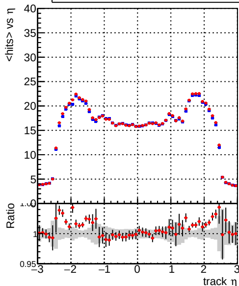
mean hits vs \eta Legend: — DQM_TT_mkFit-DQM_original — DQM_TT_mkFit-DQM_updated
