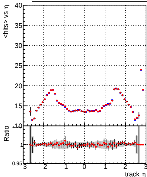
mean hits vs \eta Legend: DQM_TT_mkFit-DQM_original (blue line), DQM_TT_mkFit-DQM_updated (red line)
