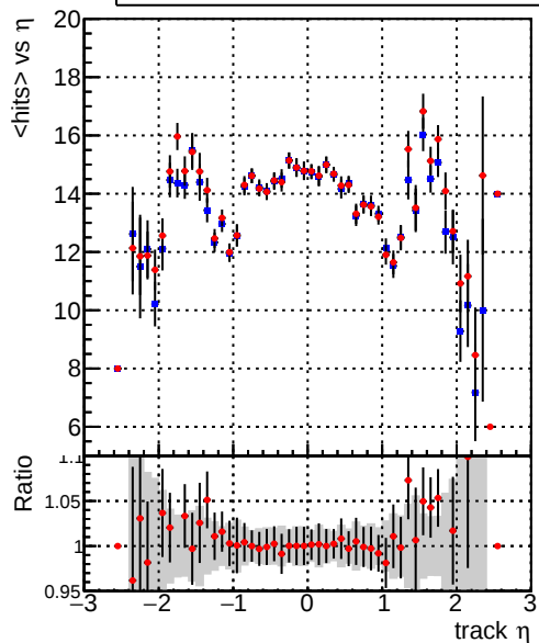
mean hits vs \eta Legend: — DQM_TT_mkFit-DQM_original — DQM_TT_mkFit-DQM_updated
