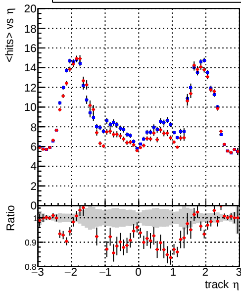
mean hit — DQM_TT_mkFit-DQM_original — DQM_TT_mkFit-DQM_updated
