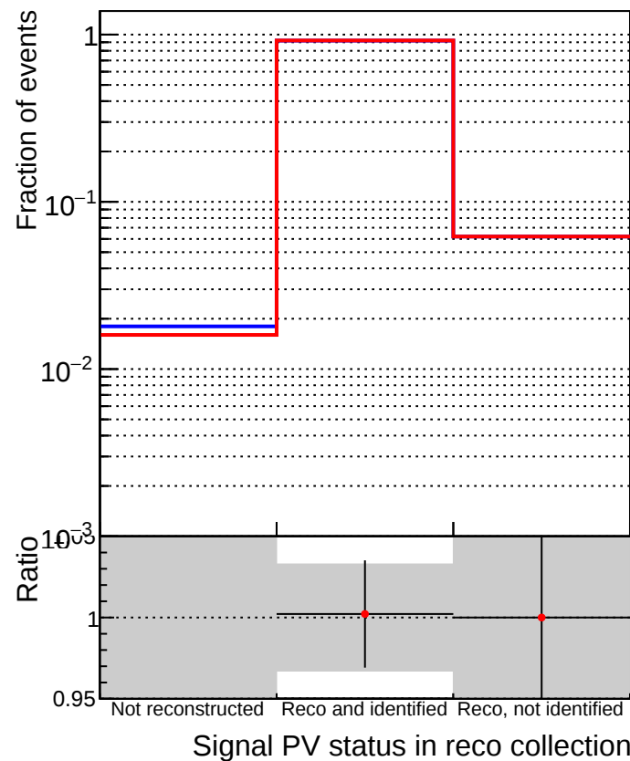
—■— DQM_TT_mkFit-DQM_original —●— DQM_TT_mkFit-DQM_updated
