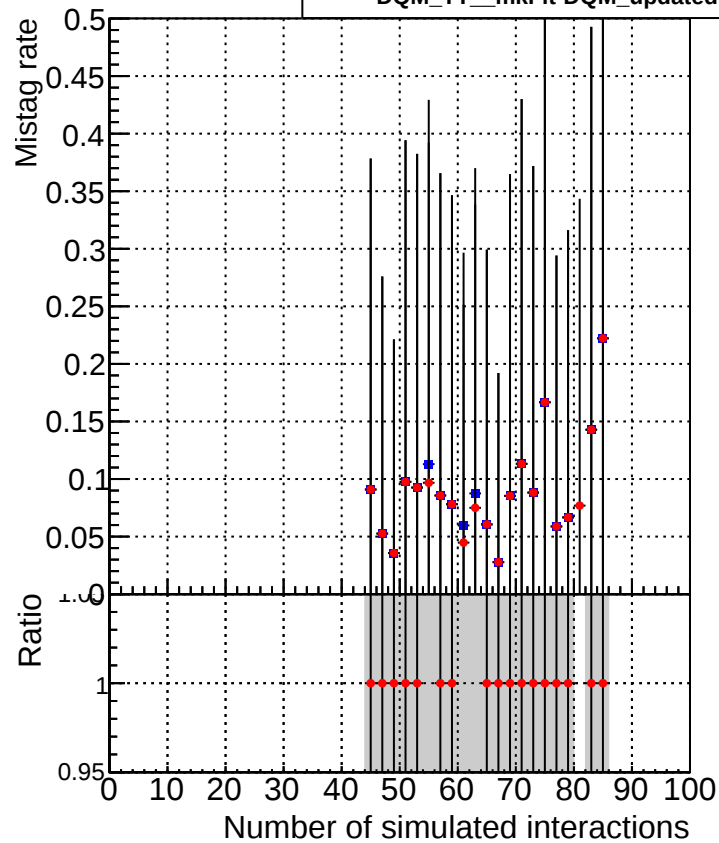
—■— DQM_TT_mkFit-DQM_original —●— DQM_TT_mkFit-DQM_updated
