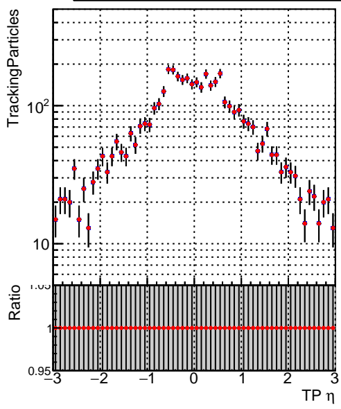
N of simulated tracks vs \eta —●— DQM_TT_mkFit-DQM_original —●— DQM_TT_mkFit-DQM_updated
