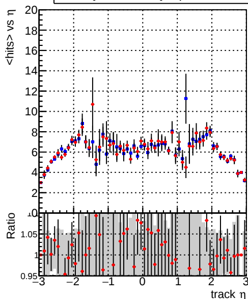
mean hits Legend: — DQM_TT_mkFit-DQM_original, — DQM_TT_mkFit-DQM_updated
