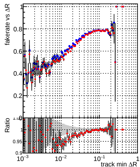
—●— DQM_TT_mkFit-DQM_original —●— DQM_TT_mkFit-DQM_updated
