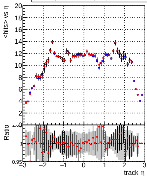
— DQM_TT_mkFit-DQM_original — DQM_TT_mkFit-DQM_updated
