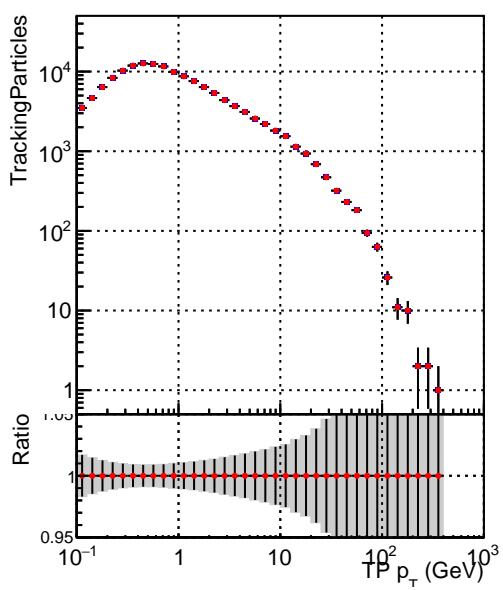
Legend: DQM_TT_mkFit-DQM_original (blue squares), DQM_TT_mkFit-DQM_updated (red stars)
