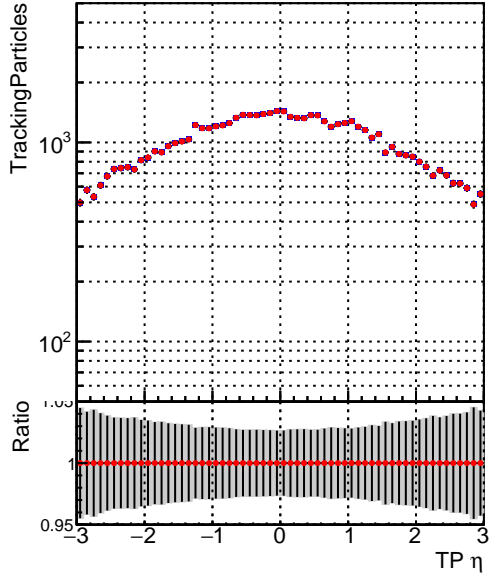
Legend: DQM_TT_mkFit-DQM_original (blue squares), DQM_TT_mkFit-DQM_updated (red stars)
