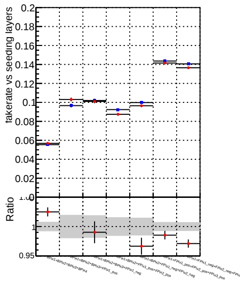
Fake rate vs. —●— DQM TT mkFit-DQM_original —●— DQM TT mkFit-DQM_updated
