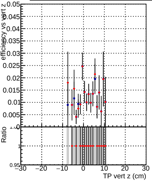
Efficiency vs TP vert z (cm) Legend: DQM_TT_mkFit-DQM_original (blue squares) DQM_TT_mkFit-DQM_updated (red stars)
