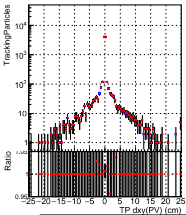
DQM_TT_mkFit-DQM_updated
