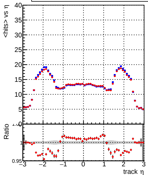
mean hits Legend: DQM_TT_mkFit-DQM_original (blue line), DQM_TT_mkFit-DQM_updated (red line)
