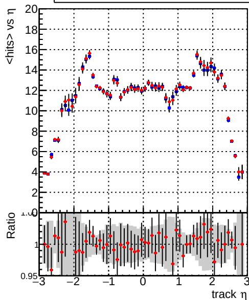
mean hits — DQM_TT_mkFit-DQM_original — DQM_TT_mkFit-DQM_updated
