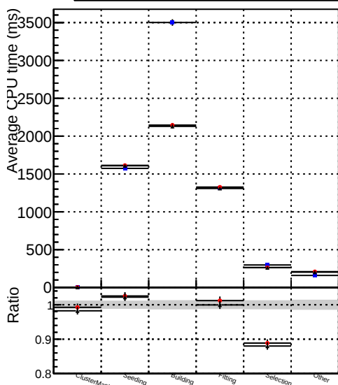
Average Legend Series DQM_V0001_R0000000001_Global_mkFitOriginal_RECO DQM_V0001_R0000000001_Global_mkFitNewALL_RECO
