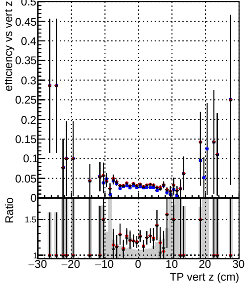
Efficiency vs vert z —●— DQM_V0001_R0000000001 Global_cmssw_RECO —●— DQM_V0001_R0000000001 Global_mkFitOriginal_RECO —●— DQM_V0001_R0000000001 Global_mkFitNewALL_RECO
