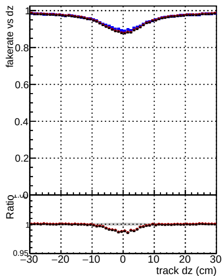
DOM V0001 R0000000001 Global cms-sw RECO Fake rate vs d Blue dots Red dots Black line Grey shaded area White area Duplicates Rate vs Dxy Blue dots Red dots Black line Grey shaded area White area Pileup rate vs dxy Blue dots Red dots Black line Grey shaded area White area
